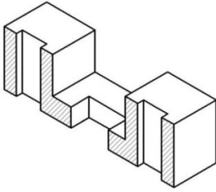
Full section (Figure: 5.4-1)
