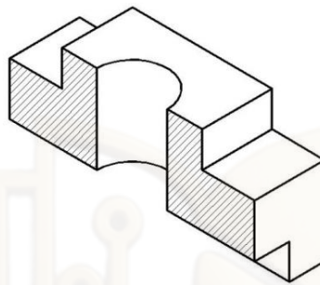
Full section (Figure: 5.4-2)
