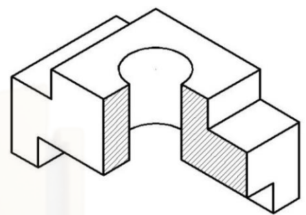
Half section (Figure: 5.4-2)
