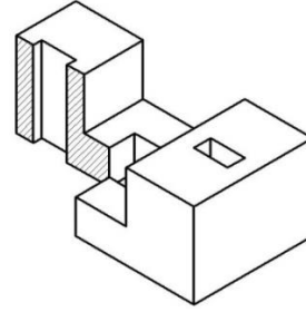
Half section (Figure: 5.4-1)
